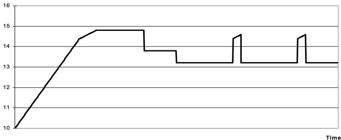
Charge voltage
