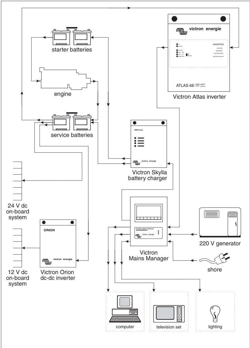
© victron energie b.v. complete VICTRON ENERGIE system drawing no.: CE320 date : 120893
